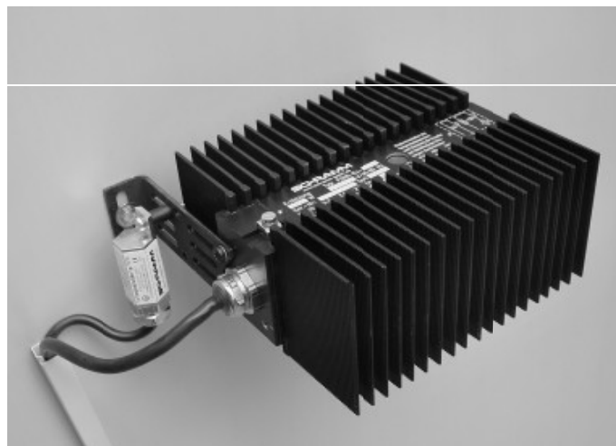
Mounting example
